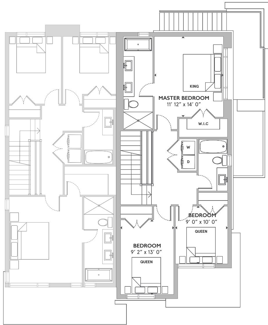
THIRD FLOOR
