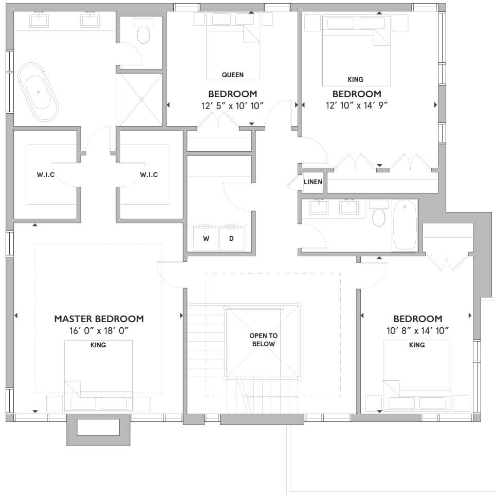
SECOND FLOOR
